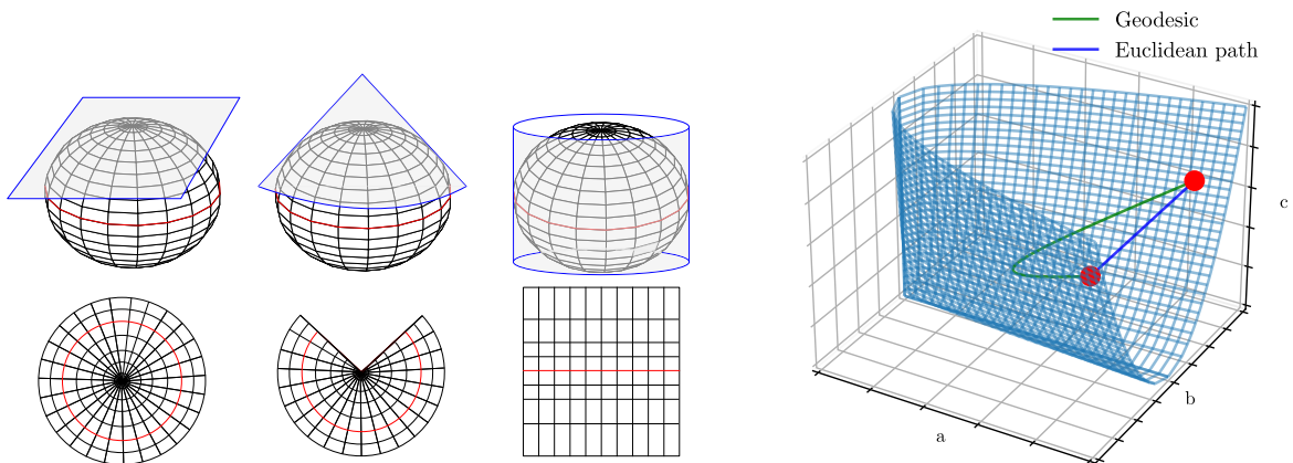
(a) Different examples of projections of the curved two-dimensional surface of a globe on a plane. All three of these projections distort in one way or another the surface. (b) The set of 2 \times 2 SPD matrices. The green path is the geodesic between two SPD matrices and the blue path is the usual Euclidean path.
